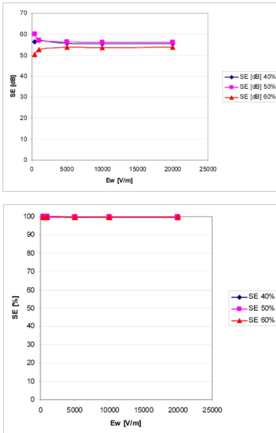
Graph 10. Electric field absorption by insulating materials as function of electric field for RH 40, 50 and 60% for Material G
