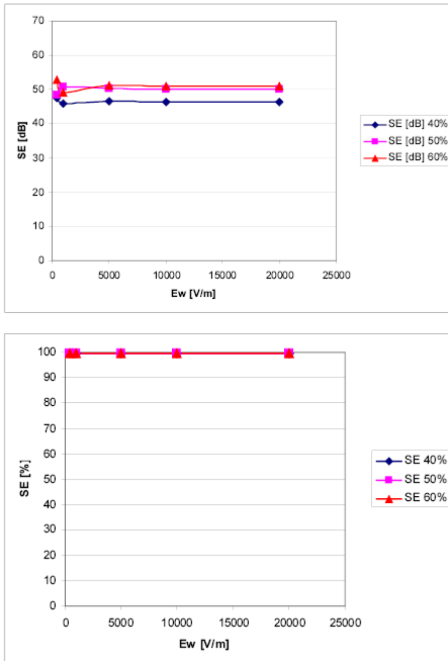
Graph 9. Electric field absorption by insulating materials as function of electric field for RH 40, 50 and 60% for Material F
