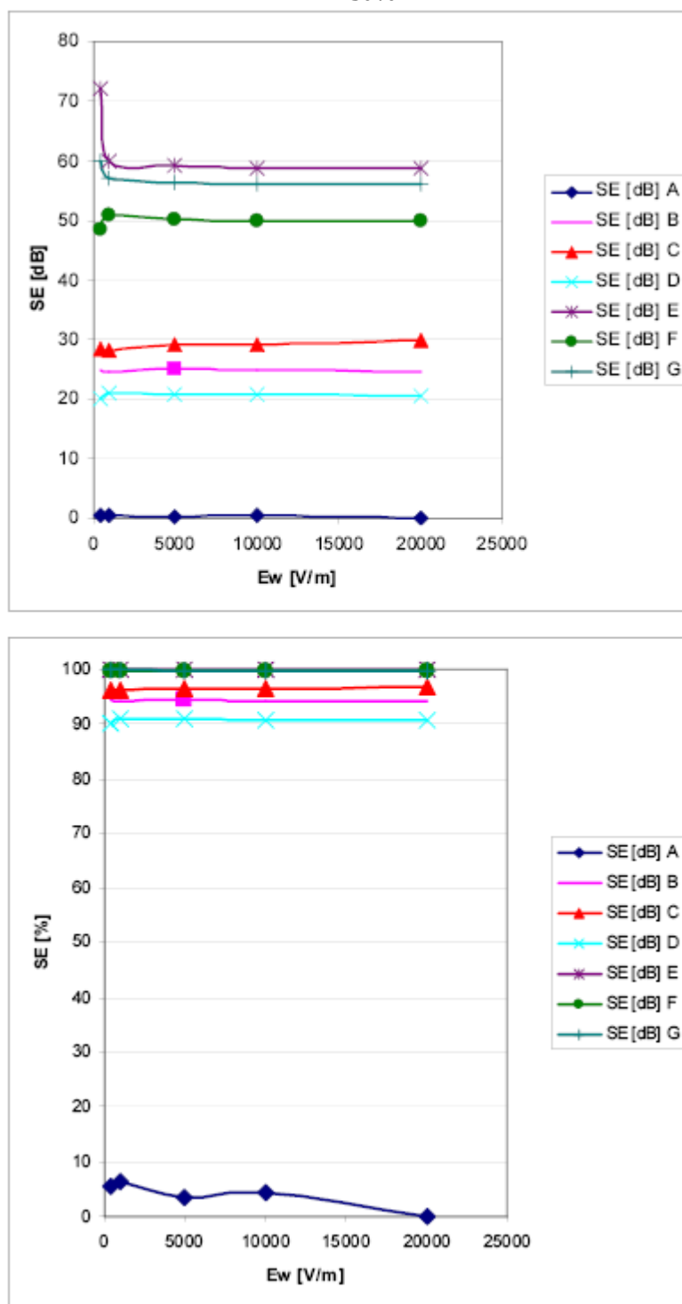
Graph 2. Electric field absorption by insulating materials as function of electric field for RH 50%
