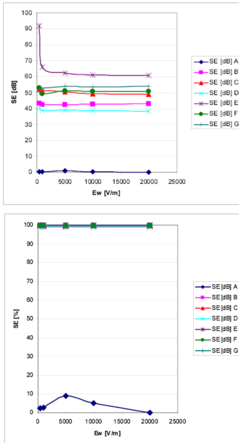
Graph 3. Electric field absorption by insulating materials as function of electric field for RH 60%
