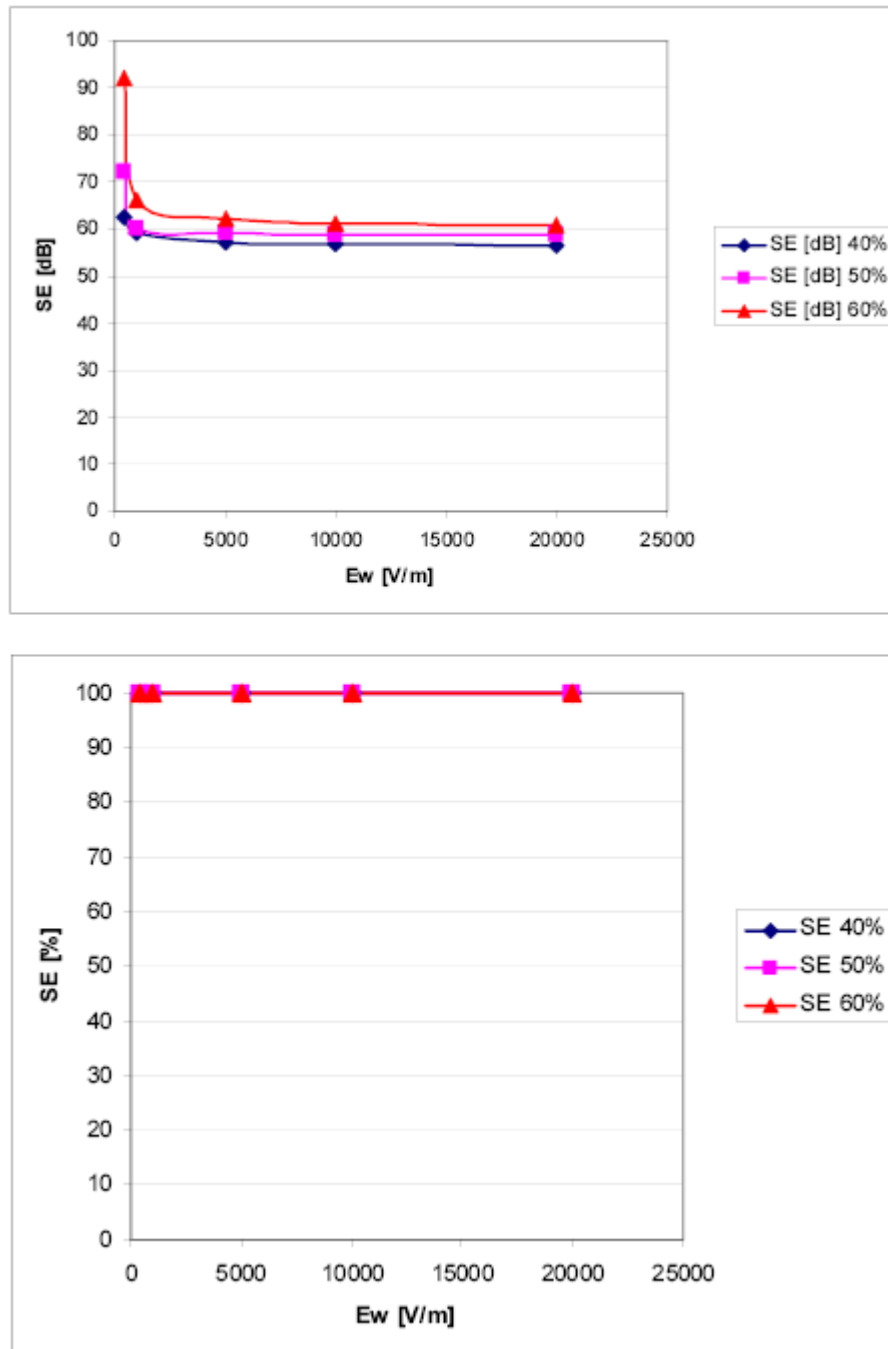
Graph 8. Electric field absorption by insulating materials as function of electric field for RH 40, 50 and 60% for Material E
