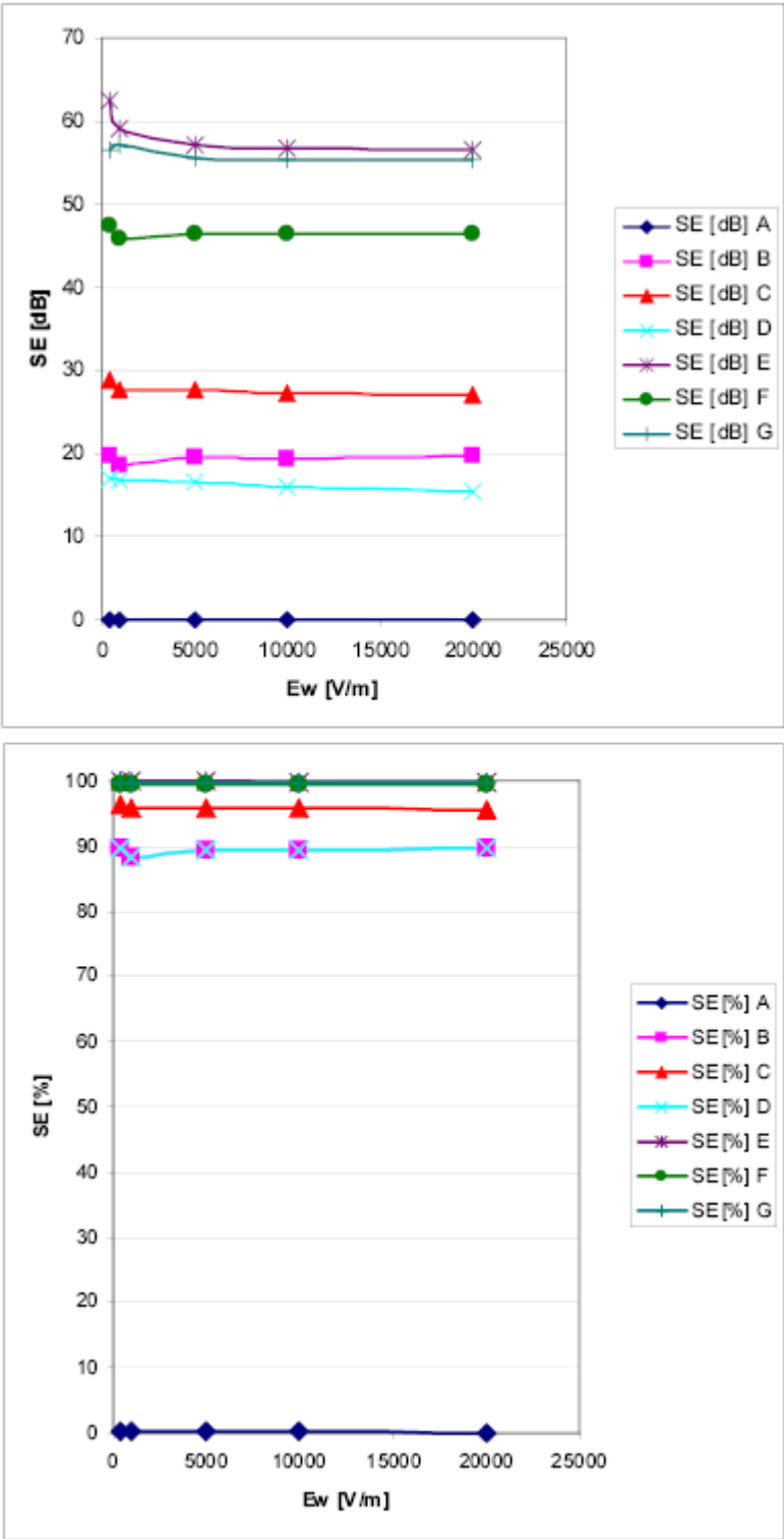
Graph 1. Electric field absorption by insulating materials as function of electric field for RH 40%
