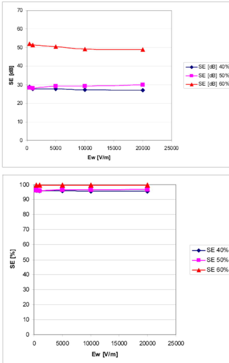
Graph 6. Electric field absorption by insulating materials as function of electric field for RH 40, 50 and 60% for Material C
